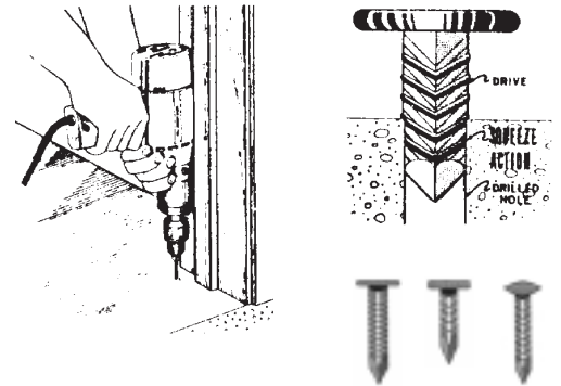
ANKR DRIVE SYSTEM
